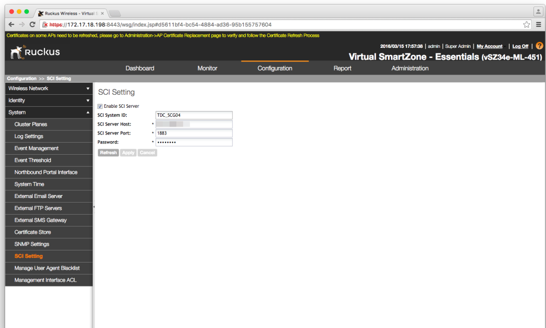
Figure 18: vSZ-E SCI settings page
